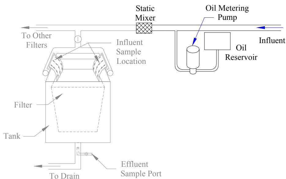
Figure 15. Schematic of Set-Up for the Continuous Dose Experiment.
