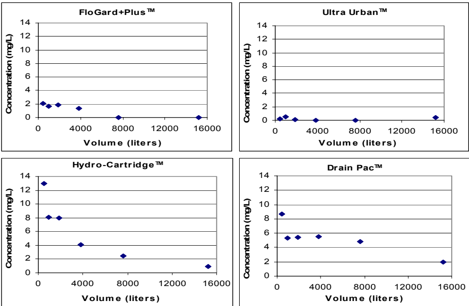
Figure 21. Graphs of Effluent Concentrations in the Clean Water Flush Test Using Method 8015.
